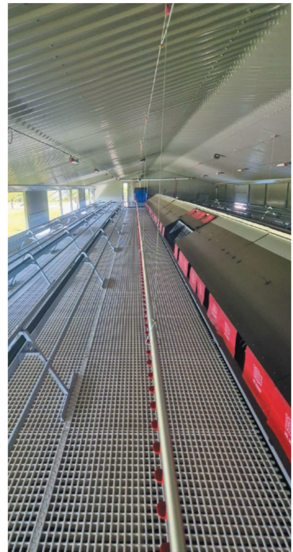
Each house measures 46m long (42.5m Bird Area + 3.5m Packing Area/Control Room) x 9m wide. The buildings have an overall height of 3.75m and are built on two galvanized steel channel skids. Each building has a large set of double doors in the Bird Area, one internal and one external personnel door, plus an additional egg pallet external door.
